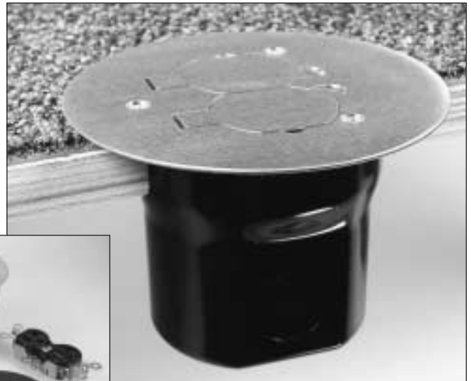
862C Residential Floor Box installed in a wood floor.
