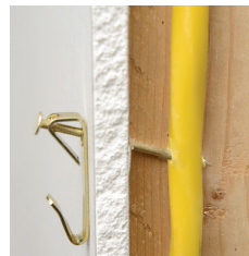
A drill bit or nail can sever the insulation of cable inside a wall.
