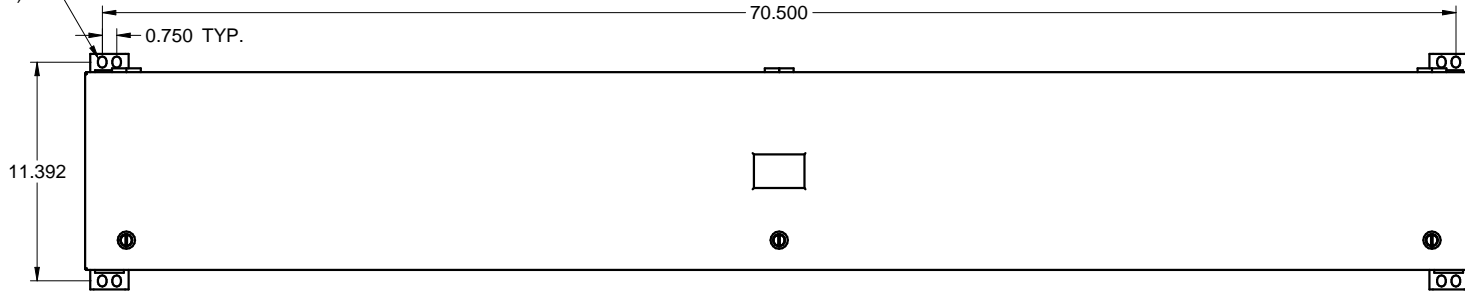
FRONT / FACE
