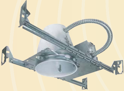
HV4S-HR01-NC 4" Remodel Housing with magnetic transformer
