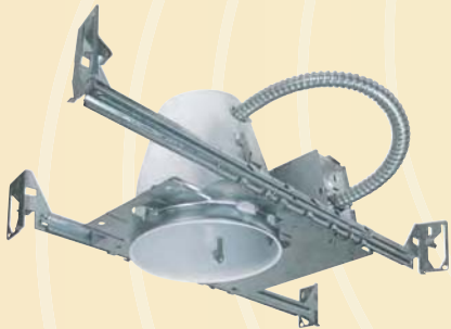
HV4-HR01-NC 4" New Construction Housing
